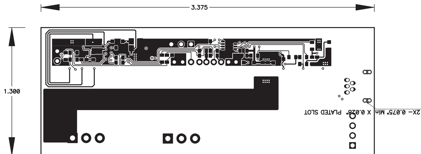
Figure 6. Bottom Layer
