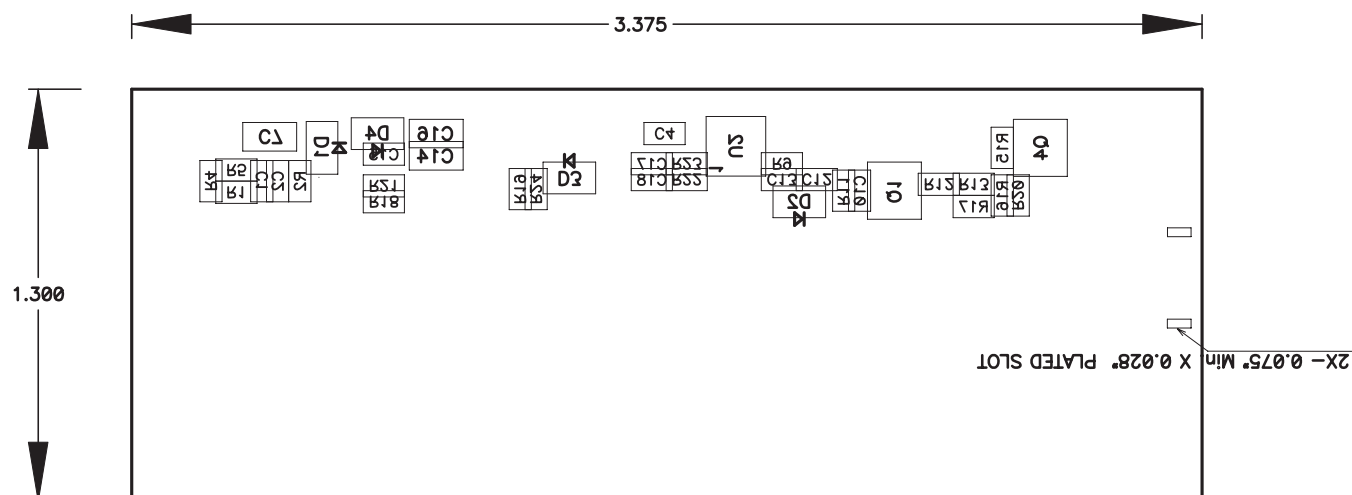
Figure 7. Bottom Assembly
