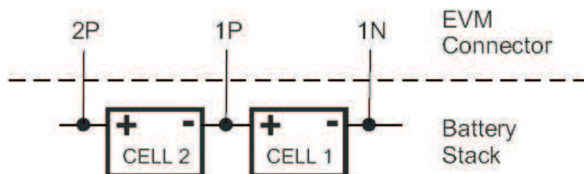
Figure 14. Connection Sequence
