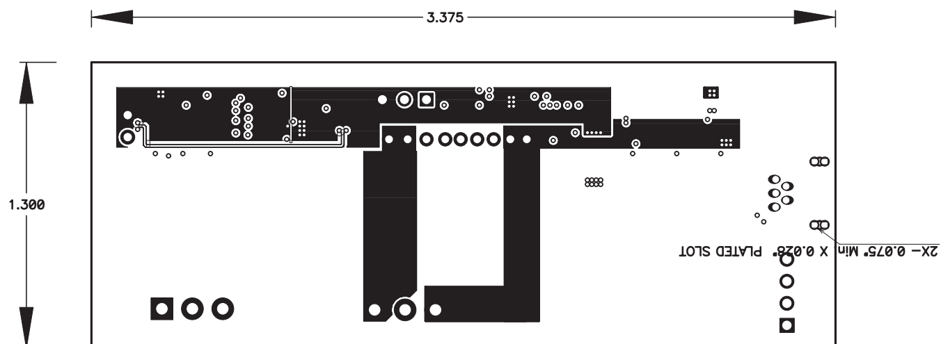
Figure 5. Internal Layer 2
