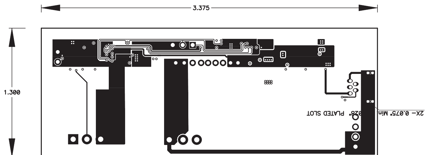
Figure 4. Internal Layer 1
