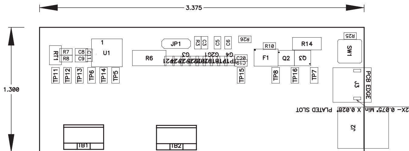
Figure 2. Top Assembly
