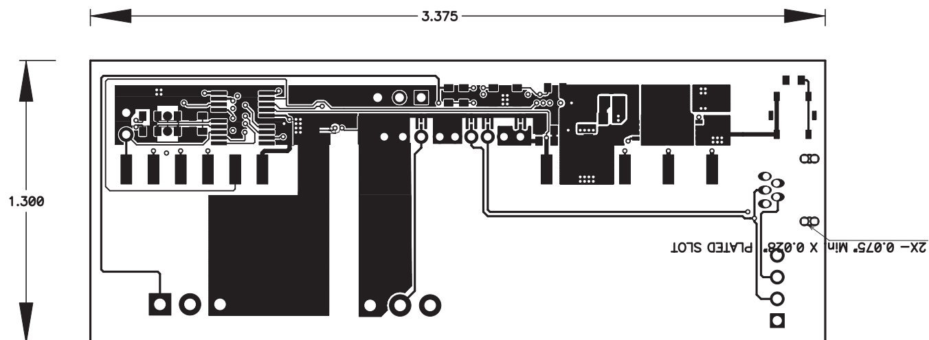
Figure 3. Top Layer
